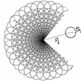
Figure 1: (Top) Retino-cortical log-polar transformation. (Bottom) Arrangement of the receptive fields in the retinal model.
