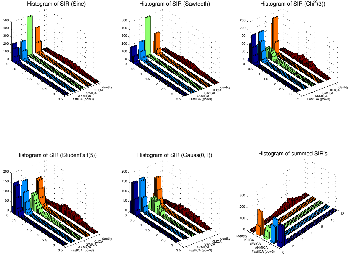
Figure 3: Histograms of SIR values for 500 ICA trials. Source-to-interference ratio (SIR) is shown for each source and for all sources (sum of SIRs).
