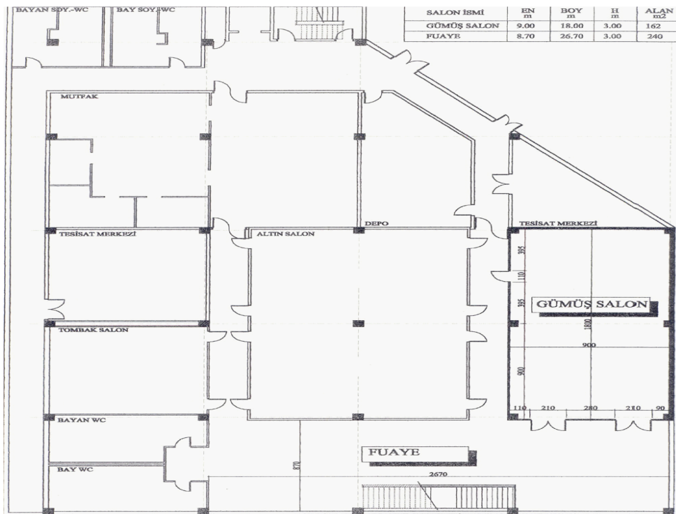
Fig. 2: The plan of the Talya Convention Center ground floor: Altin, Gumus and Tombak Halls.
