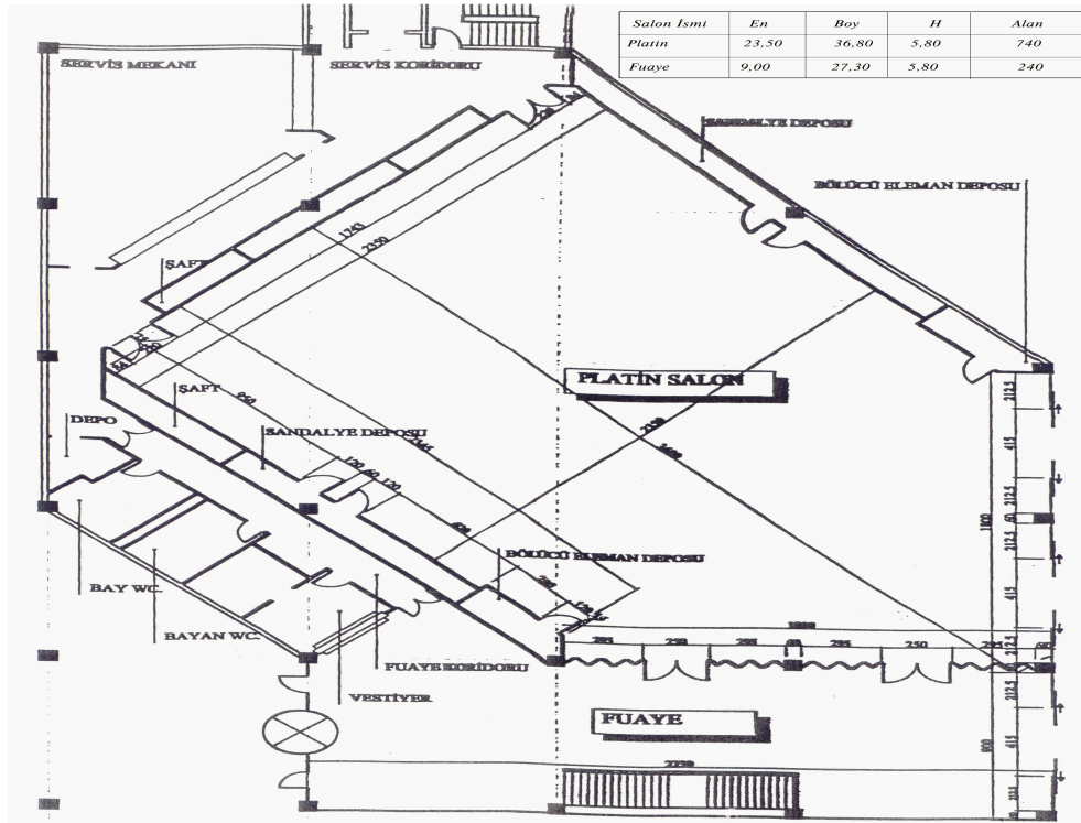
Fig. 1: The plan of the Talya Convention Center roof floor: Fuaye and Platin Hall.
